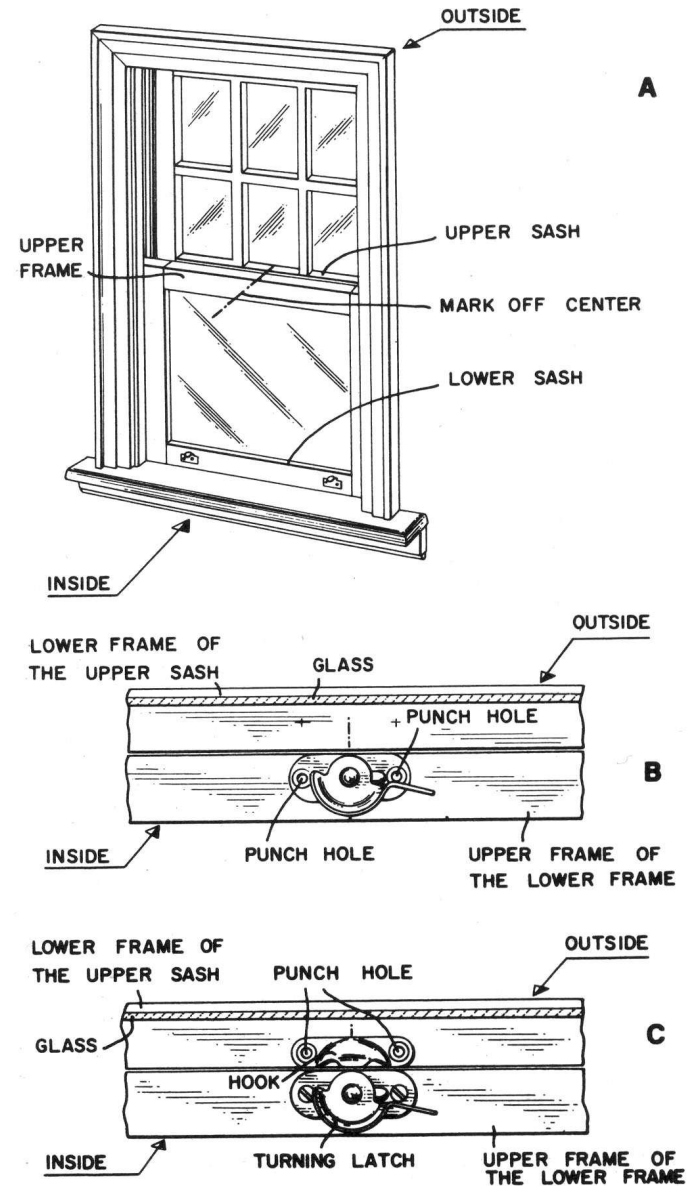
Figure 24. To Lock a Window
