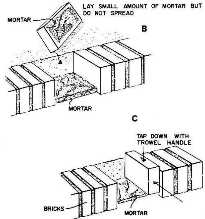
Figure 97. How To Lay New Brick
